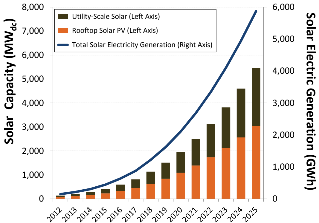
Figure ES-1. Potential Solar Photovoltaic Market Growth in Oregon Through 2025
