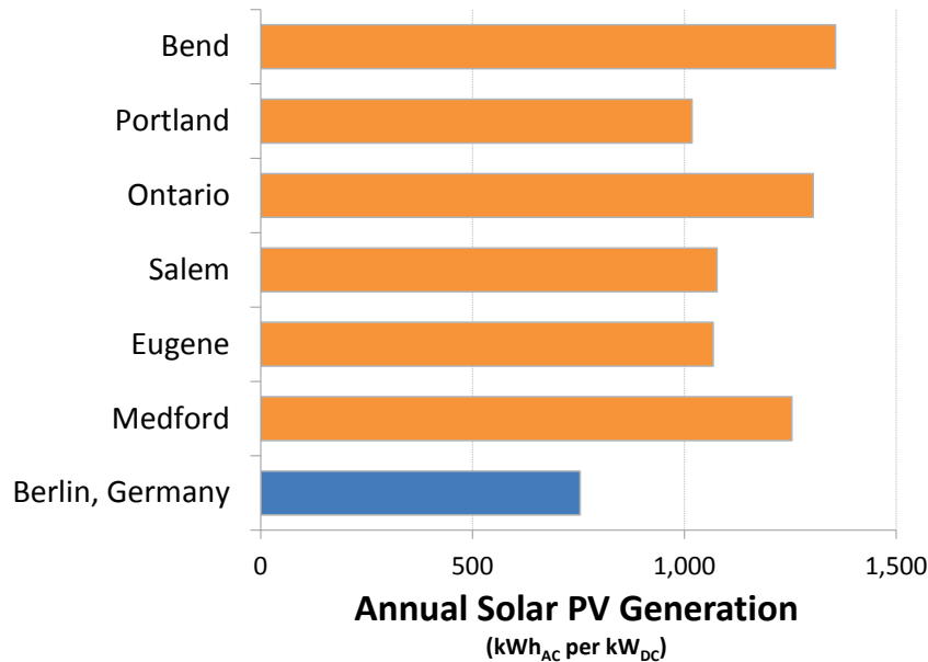
Figure 2: Solar Energy Resources Compared 4
