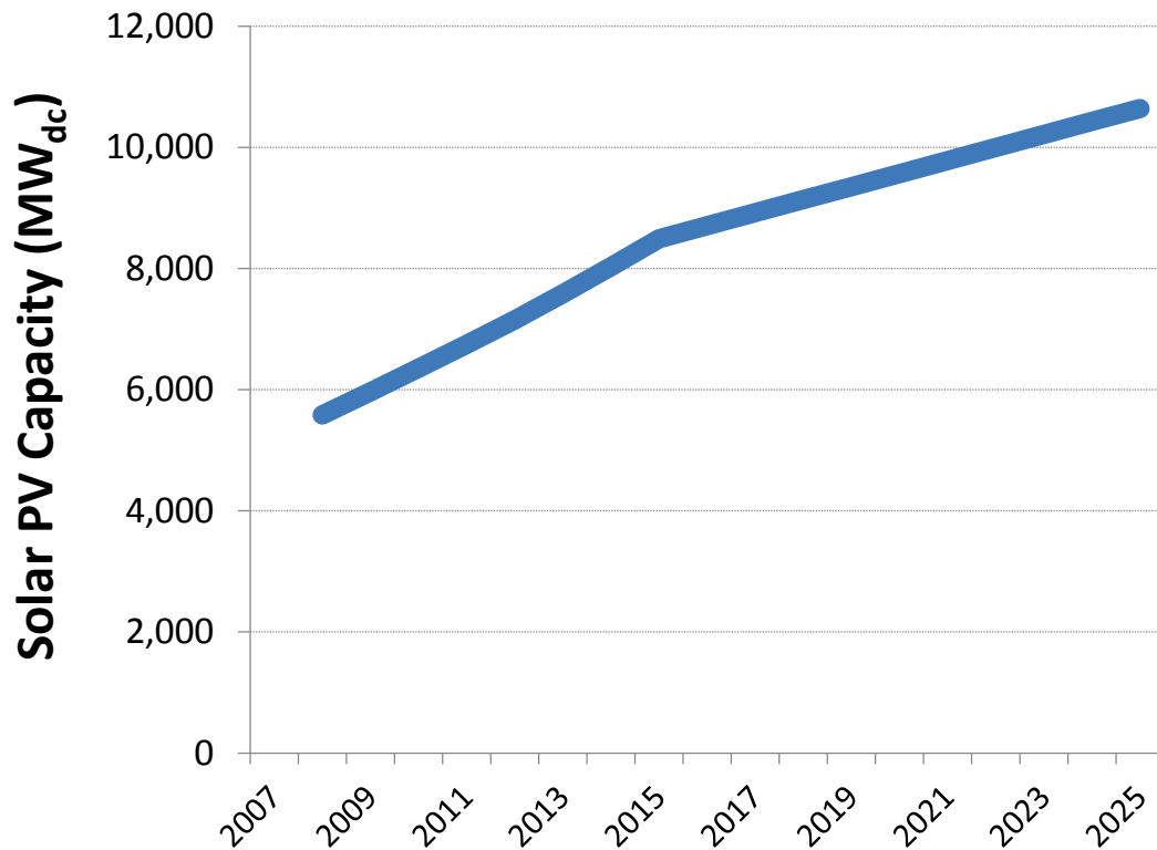
Figure 3: Total Technical Rooftop Solar PV Potential in Oregon Based on Available Rooftop Area 20
